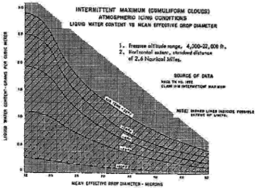
Figure 4 - Intermittent maximum (cumuliform clouds) atmospheric icing conditions.
