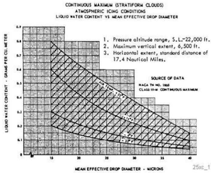
Figure 1 - Continuous maximum (stratiform clouds) atmospheric icing conditions.
