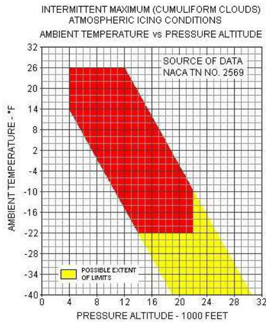
Figure 5 - Intermittent maximum (cumuliform clouds) atmospheric icing conditions. Ambient temperature versus pressure altitude.
