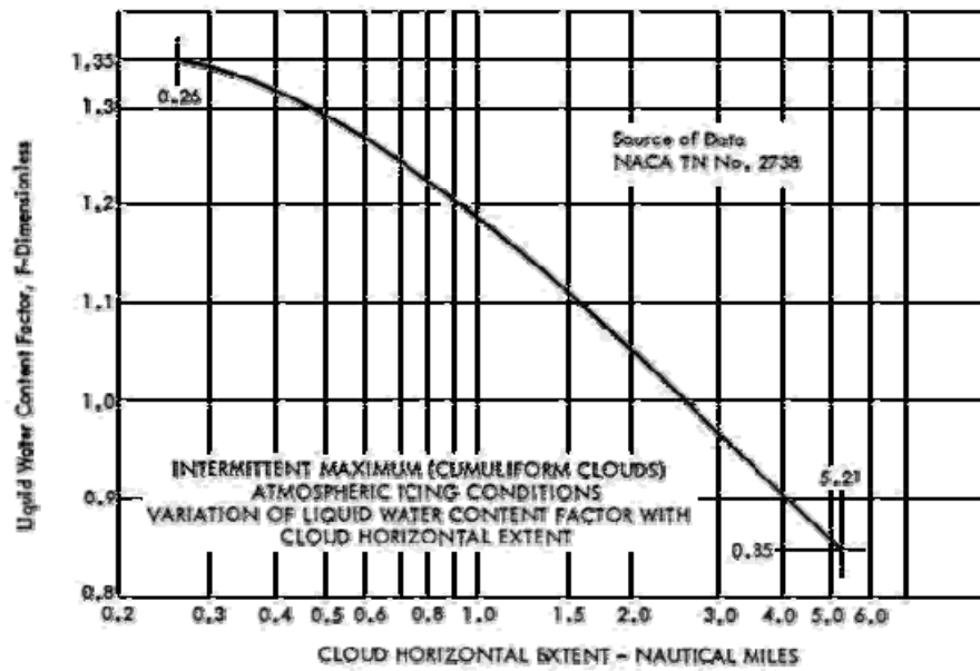
Figure 6 - Intermittent maximum (cumuliform clouds) atmospheric icing conditions.
