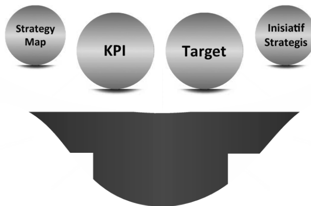
Gambar 2. Objek Cascading
